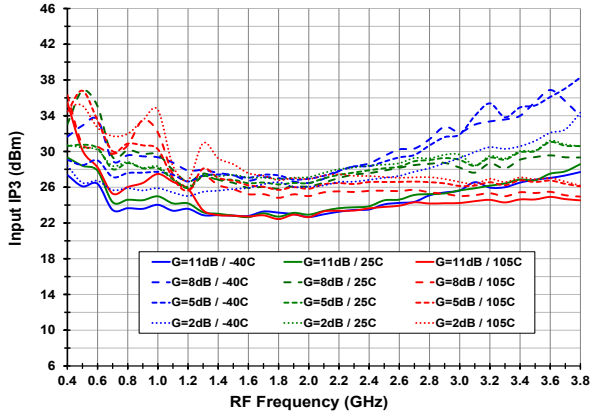
IIP3 vs. Temperature and Gain Setting
