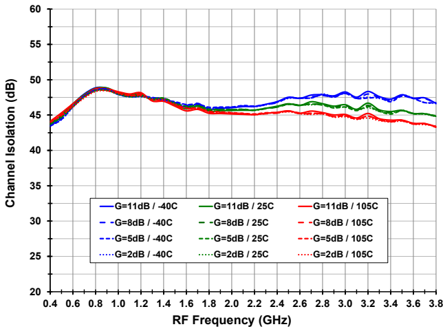
Channel Isolation vs. Temperature and Gain Setting
