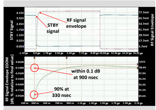
STBY Settling Time
