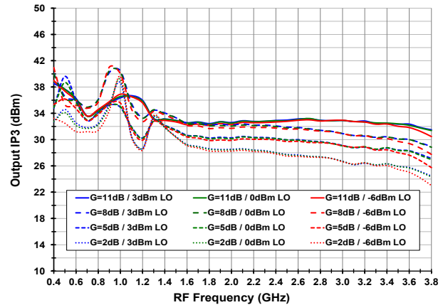
OIP3 vs. LO Power and Gain Setting (Vcc = 3.15, Tcase = 105C)
