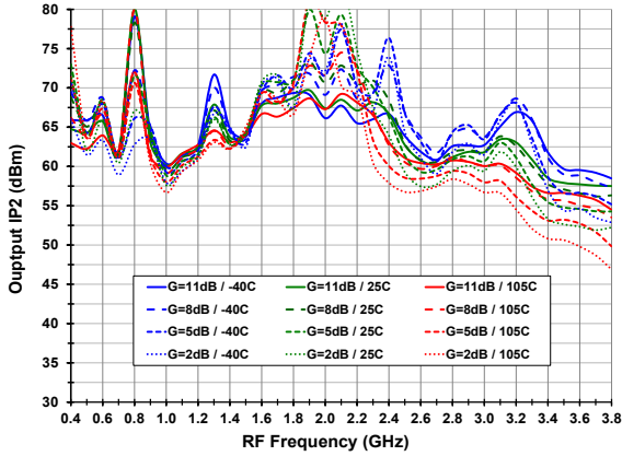
Output IP2 vs. Temperature and Gain Setting
