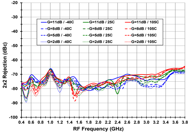
2x2 Rejection vs. Temperature and Gain Setting
