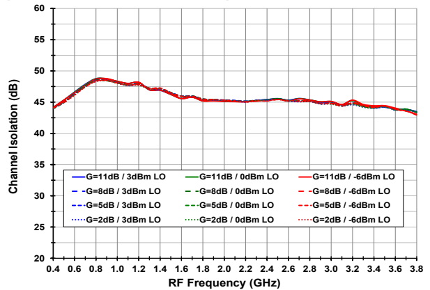
Channel Isolation vs. LO Power and Gain Setting (Vcc = 3.15, Tcase = 105C)
