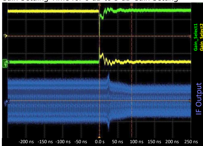
Gain Settling Time for 8 dB to 5 dB Gain Setting
