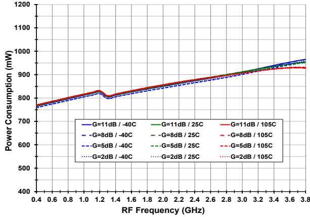
Power Consumption vs. Temperature and Gain Setting
