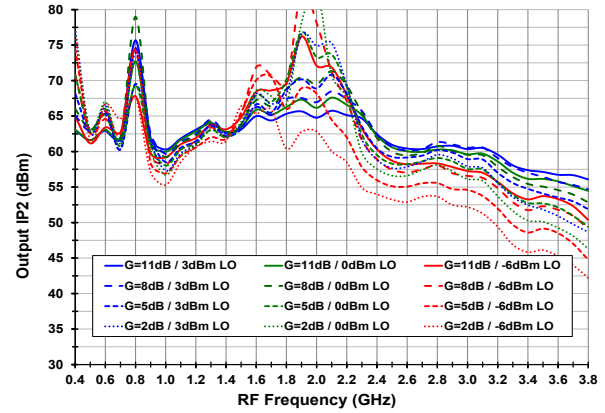
Output IP2 vs. Temperature and Gain Setting (Vcc = 3.15, Tcase = 105C)
