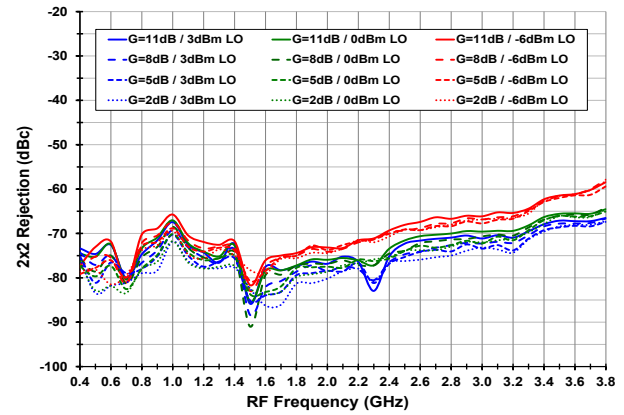
2x2 Rejection vs. LO Power and Gain Setting (Vcc = 3.15, Tcase = 105C)
