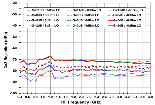
3x3 Rejection vs. LO Power and Gain Setting (Vcc = 3.15, Tcase = 105C)
