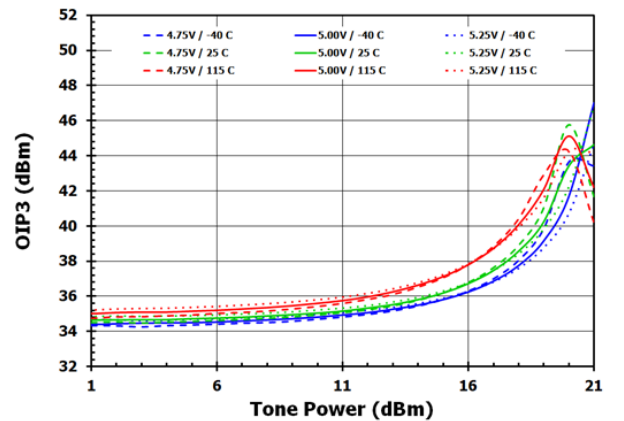
Figure 7. OIP3 vs Tone Power (2.6GHz)
