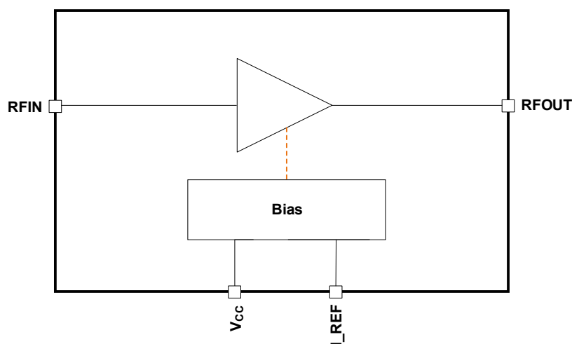
Figure 1. Block Diagram
