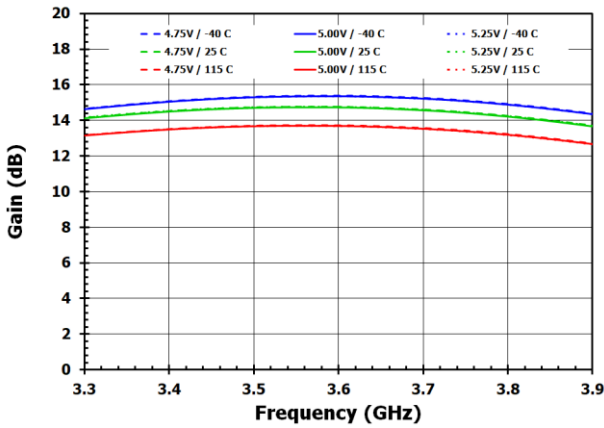
Figure 10. Gain
