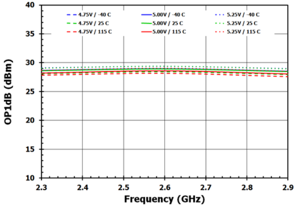
Figure 8. OP1dB (2.6GHz)
