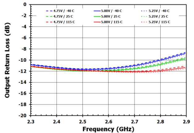
Figure 5. Output Return Loss
