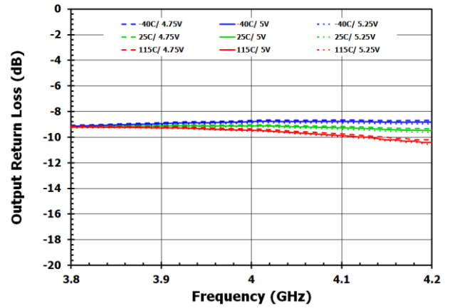
Figure 21. Output Return Loss
