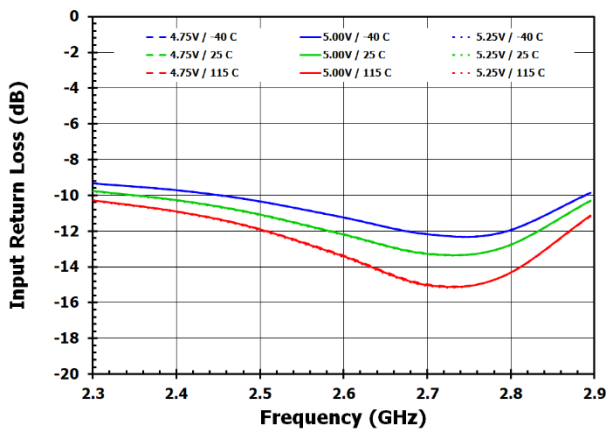
Figure 4. Input Return Loss
