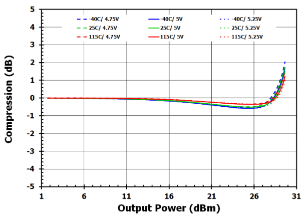
Figure 24. OP1dB (4GHz)
