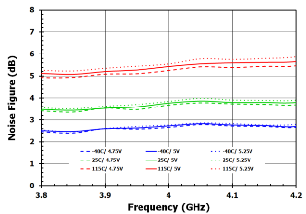
Figure 25. Noise Figure
