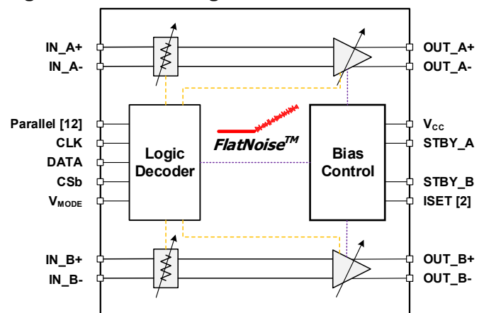
Figure 1. Block Diagram
