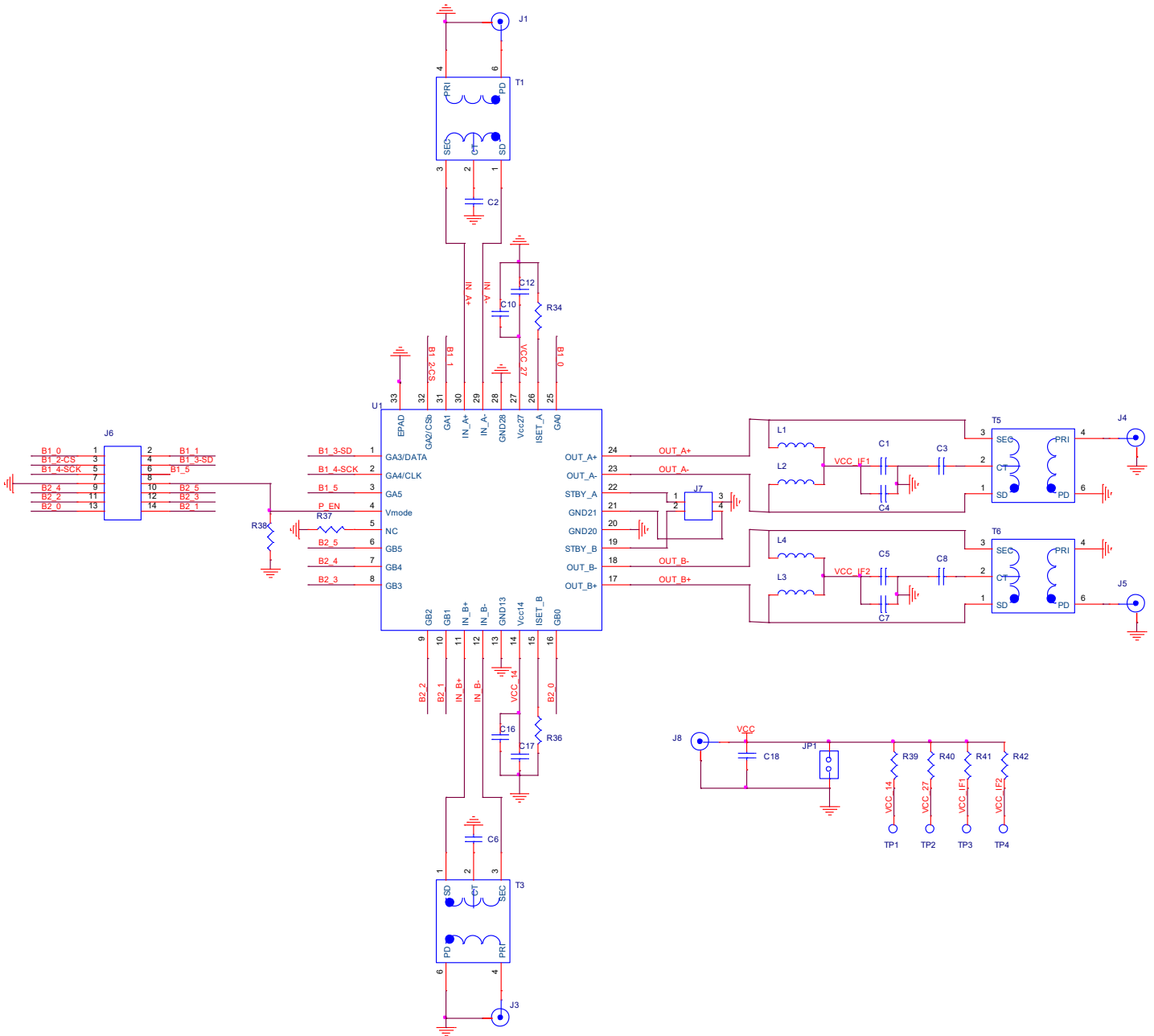
Figure 46. Electrical Schematic
