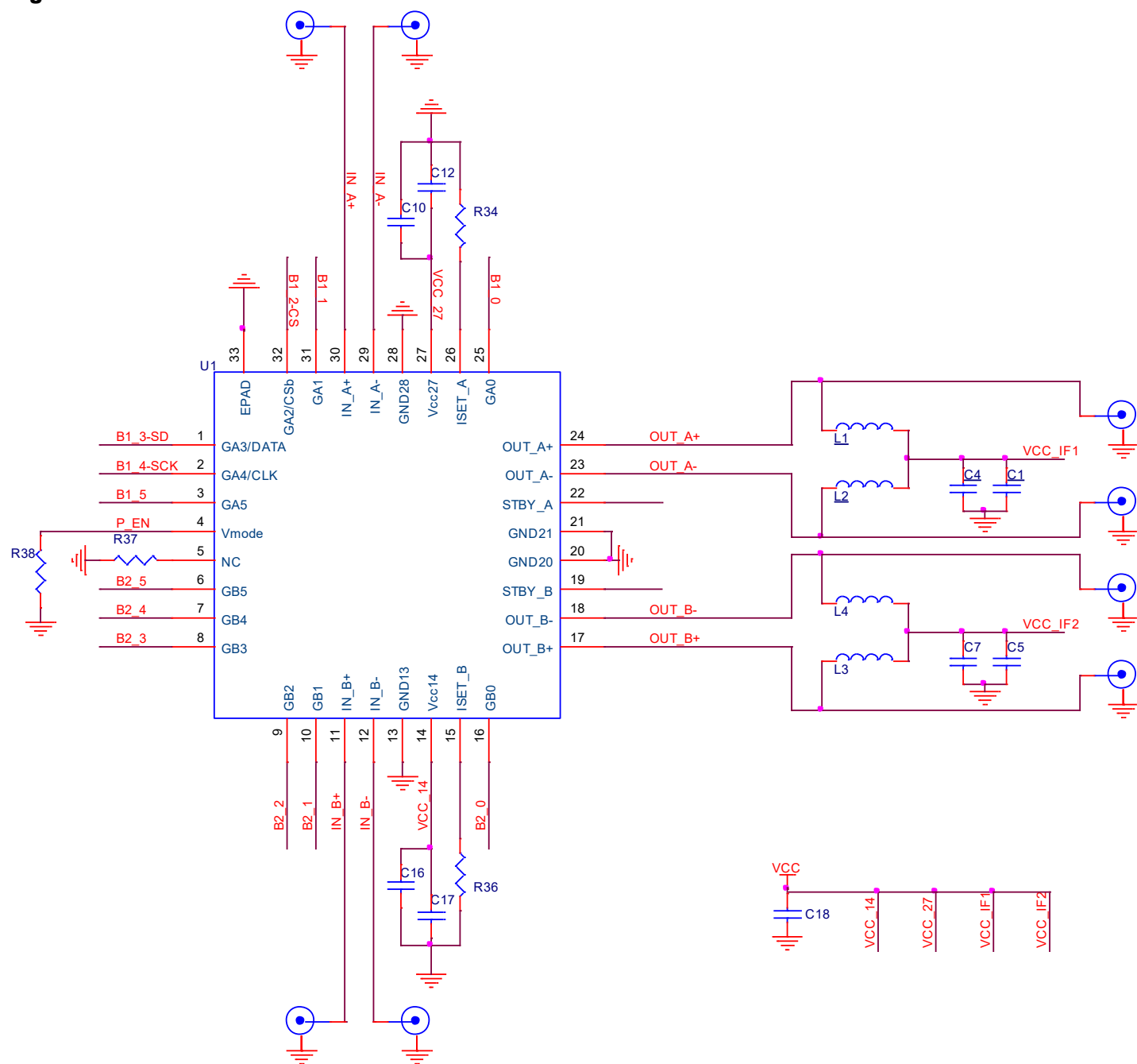
Figure 43. Electrical Schematic
