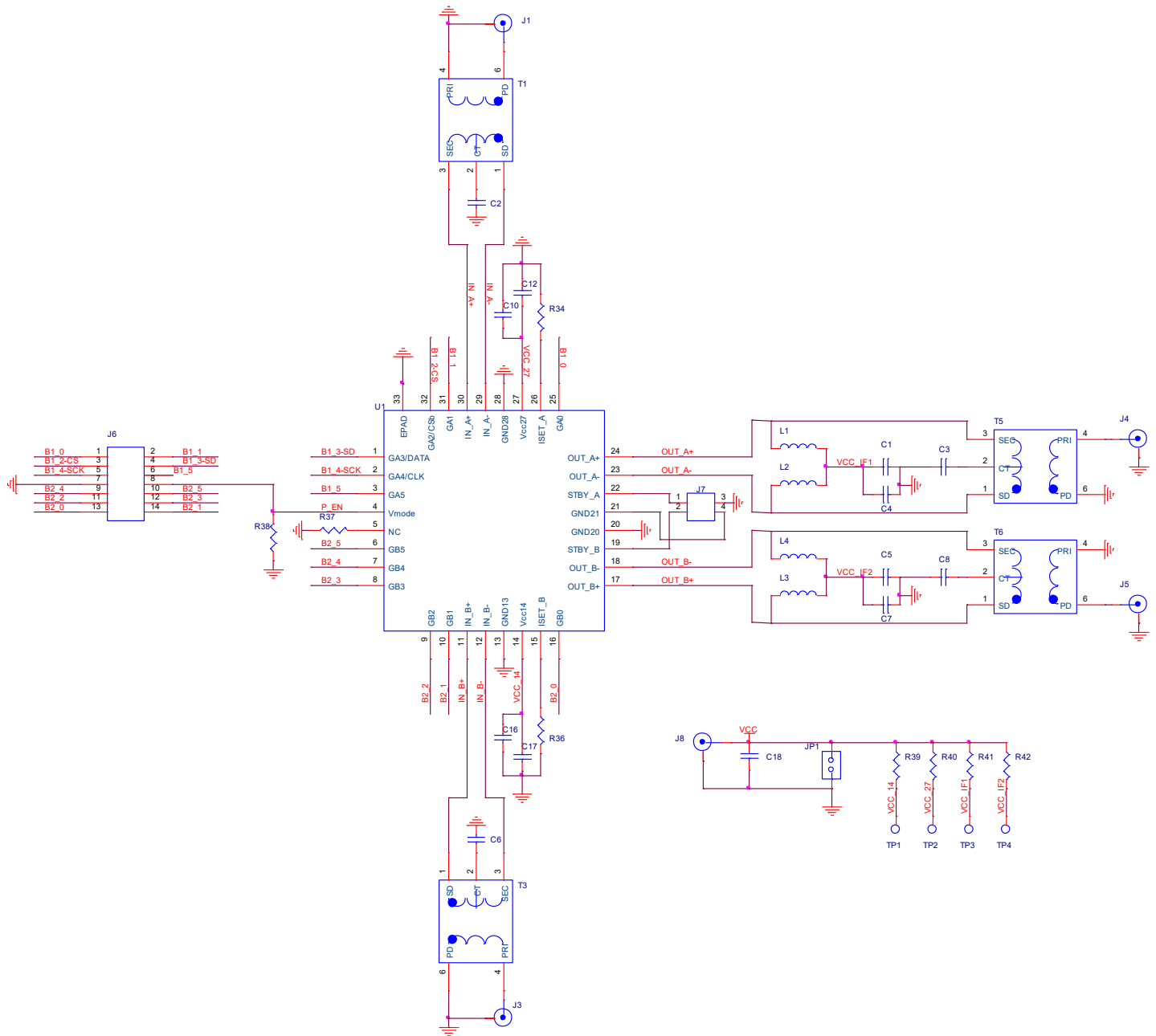
Figure 46. Electrical Schematic
