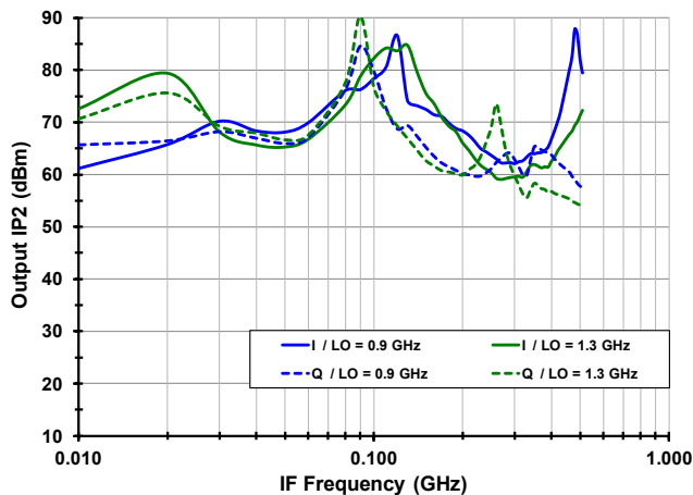
IP2o Flatness [High Side Injection, RF_X LO_A]
