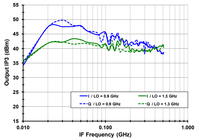
IP3o Flatness [High Side Injection, RF_Y LO_B]
