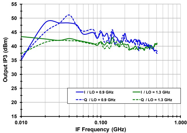
IP3o Flatness [High Side Injection, RF_X LO_A]
