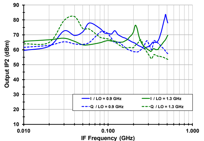
IP2o Flatness [High Side Injection, RF_Y LO_B]
