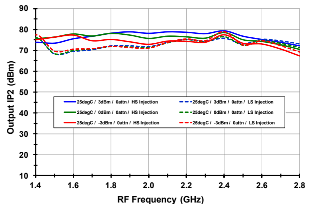
IP 2O [VS. LO LEVEL]
