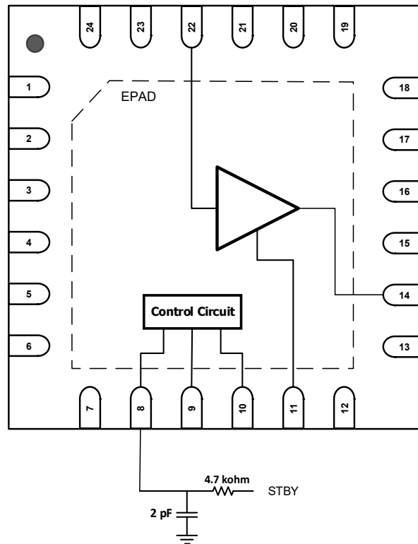
Figure 20. Control Pin Interface for Signal Integrity
