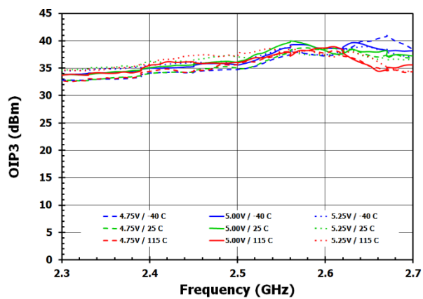
Figure 7. OIP3
