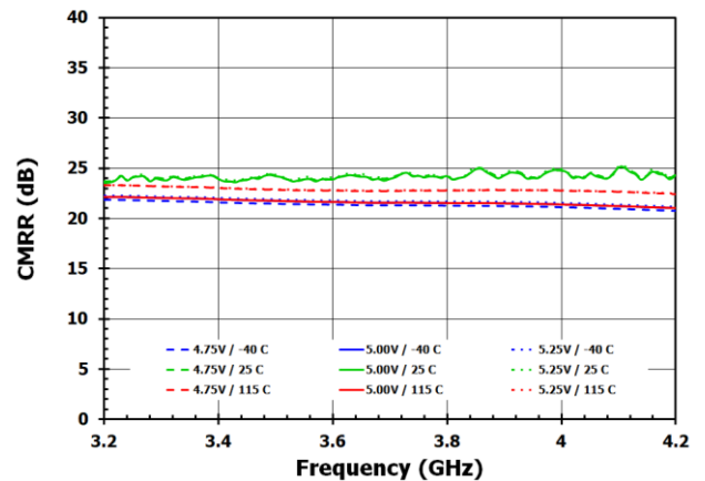
Figure 23. CMRR
