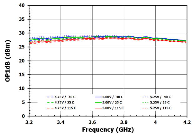
Figure 19. OP1dB
