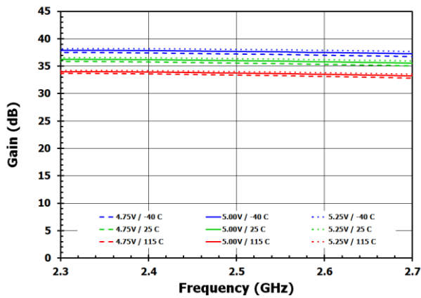
Figure 3. Gain
