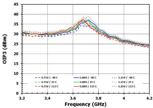
Figure 18. OIP3
