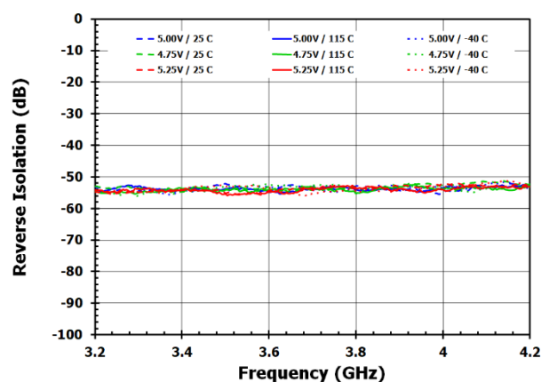
Figure 15. Reverse Isolation
