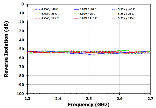
Figure 4. Reverse Isolation
