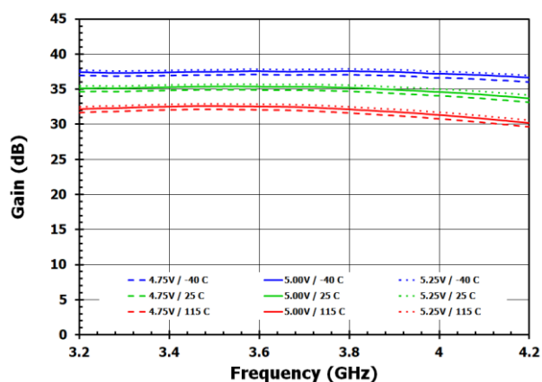
Figure 14. Gain
