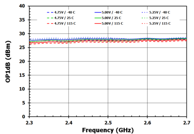
Figure 8. OP1dB
