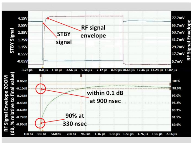
Figure 45. STBY Settling Time
