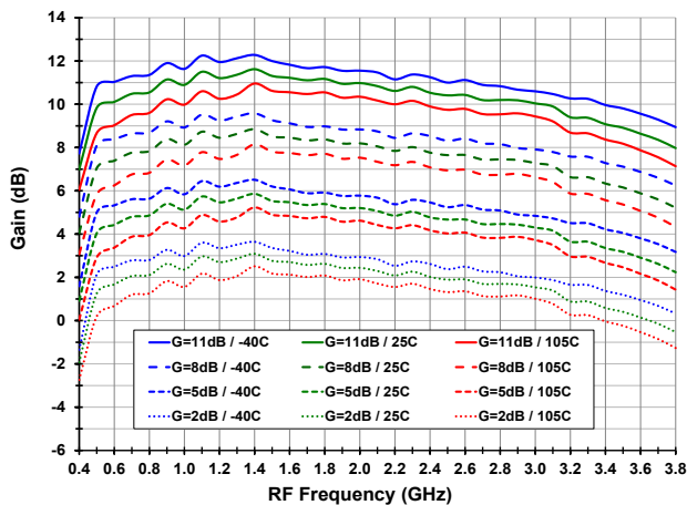
Figure 5. Gain vs. Temperature and Gain Setting
