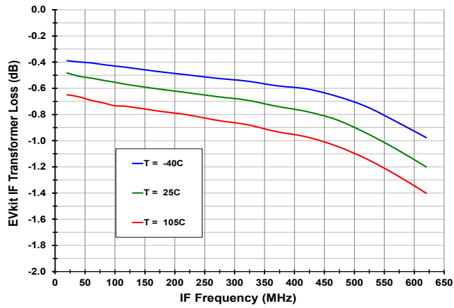
Figure 44. Evaluation Kit RF Trace Loss vs. Temperature
