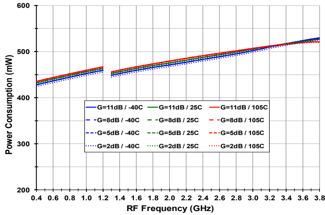
Figure 12. Power Consumption vs. Temperature and Gain Setting ( V_{CC} = 3.15 , T_{CASE} = 105^{\circ}\text{C} )
