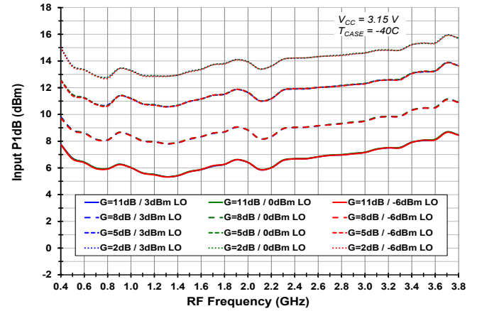
Figure 10. Input P1dB vs. LO Level and Gain Setting ( V_{CC} = 3.15 , T_{CASE} = -40^{\circ}\text{C} )
