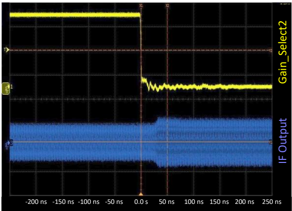
Figure 51. Gain Settling Time for 2dB to 5dB Gain Setting
