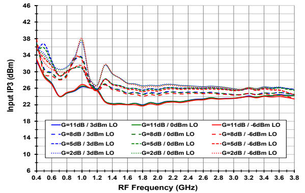
Figure 7. OIP3 vs. LO Power and Gain Setting (Vcc = 3.15, Tcase = 105°C)
