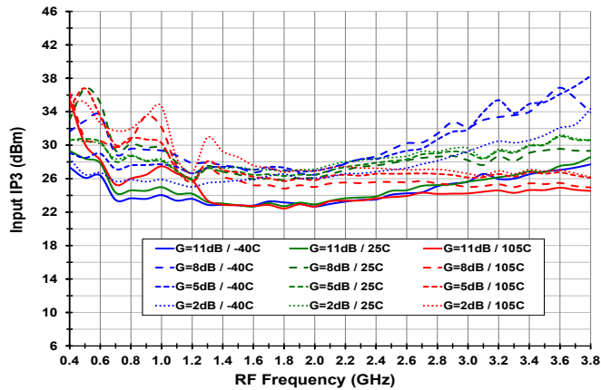
Figure 4. OIP3 vs. Temperature and Gain Setting
