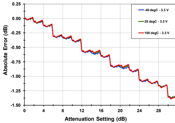
INL [900 MHz]
