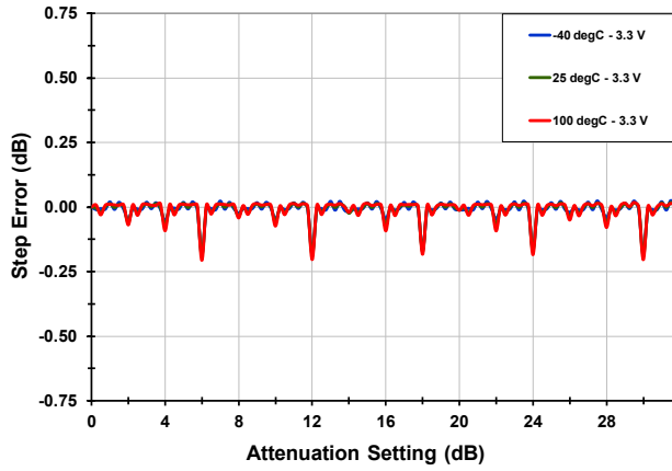
DNL [900 MHz]
