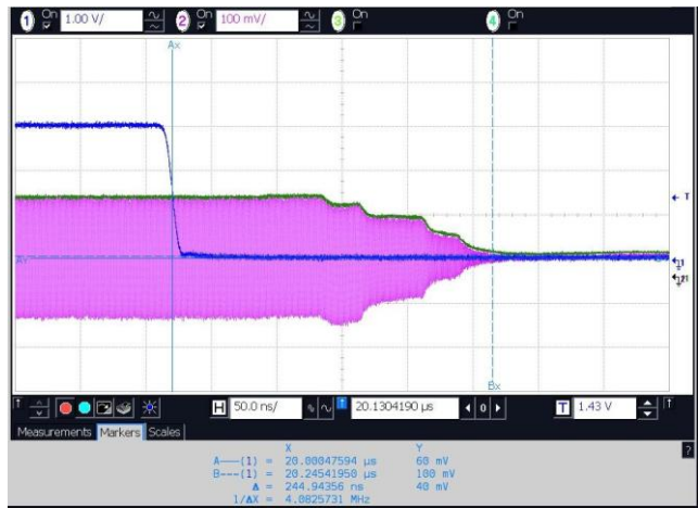
Figure 17. TOFF Switching Time
