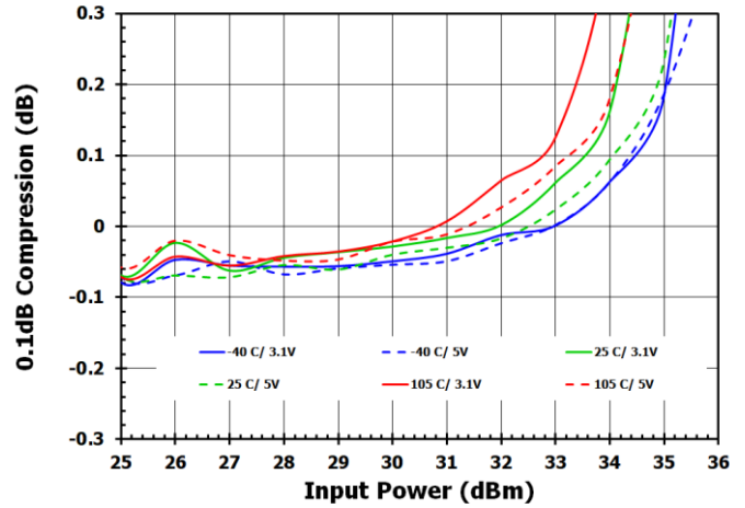
Figure 12. P0.1dB Compression (50MHz)
