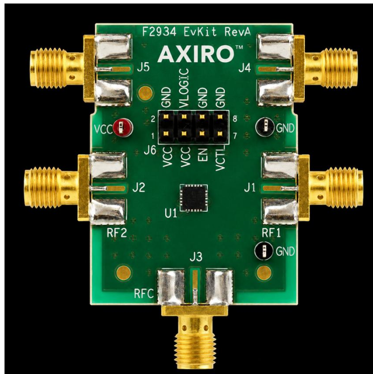
Figure 19. Evaluation Board – Top View
