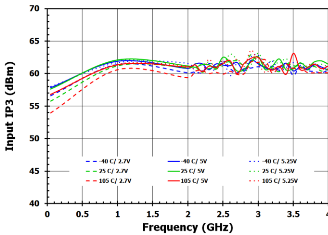
Figure 11. Input IP3
