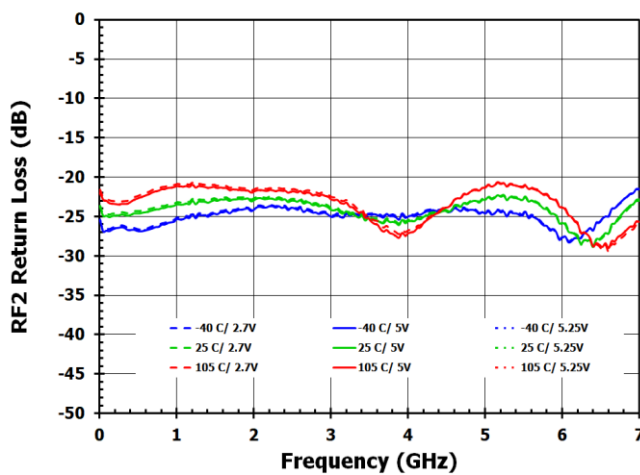
Figure 6. RF2 Return Loss
