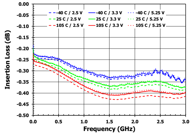
Figure 5. RF2 to RFC Insertion Loss
