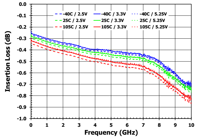
Figure 15. RF2 to RFC Insertion Loss
