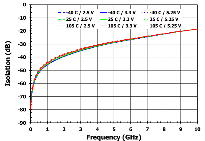
Figure 19. RF1 to RF2 Isolation [RF2 On State]
