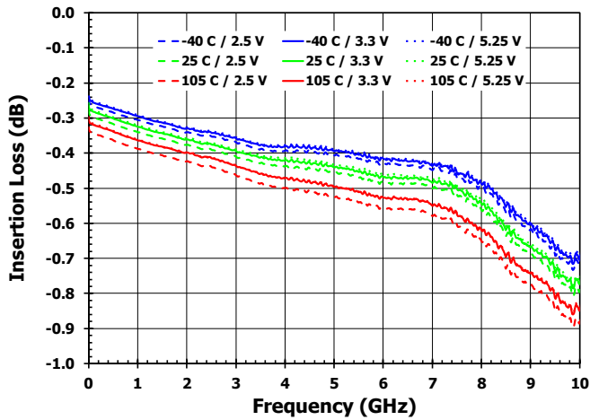
Figure 14. RF1 to RFC Insertion Loss
