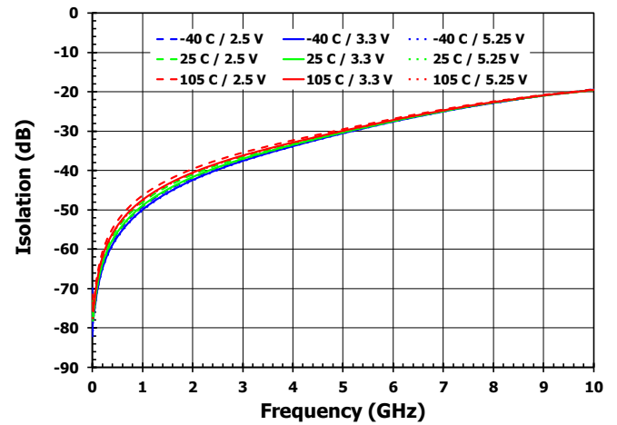
Figure 17. RF2 to RFC Isolation [RF1 On State]
