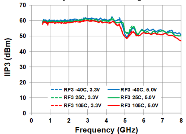
Figure 33. RF3 IIP3 vs. Frequency over Temperature and Voltage
