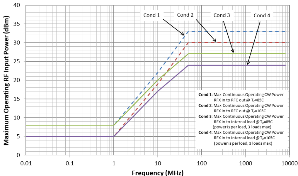
Figure 3. Maximum CW RF Input Operating Power vs. RF Frequency
