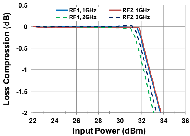
Compression [1 GHz, 2 GHz, RF1, RF2]
