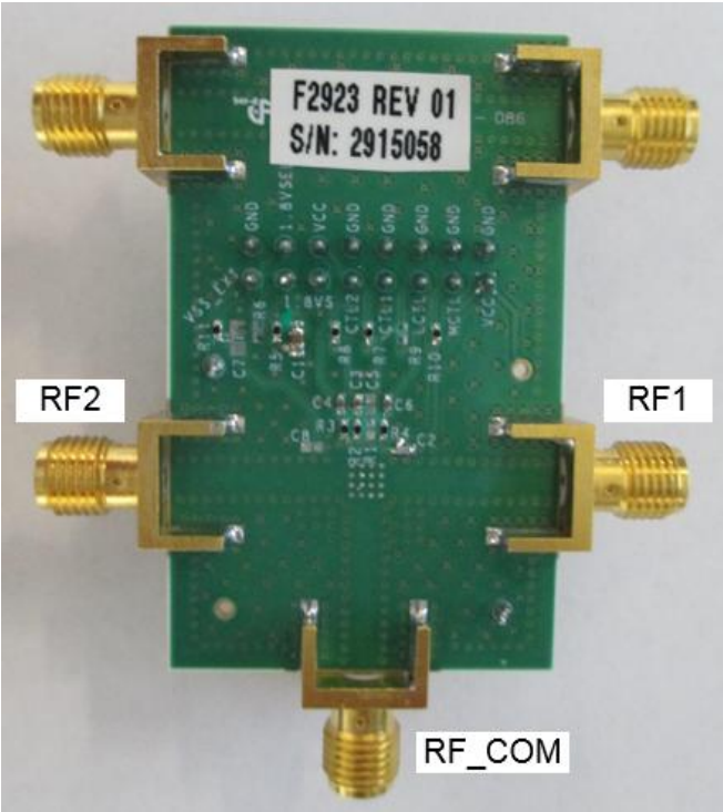
Bottom View
