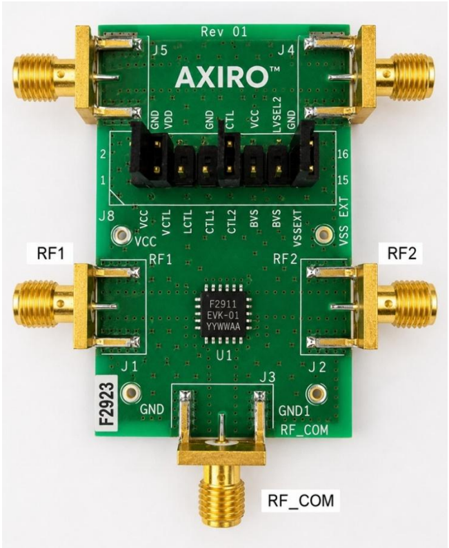
Top View
