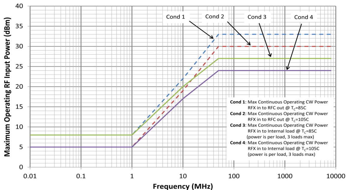
Figure 1 - MAXIMUM RF OPERATING INPUT POWER vs. RF FREQUENCY
