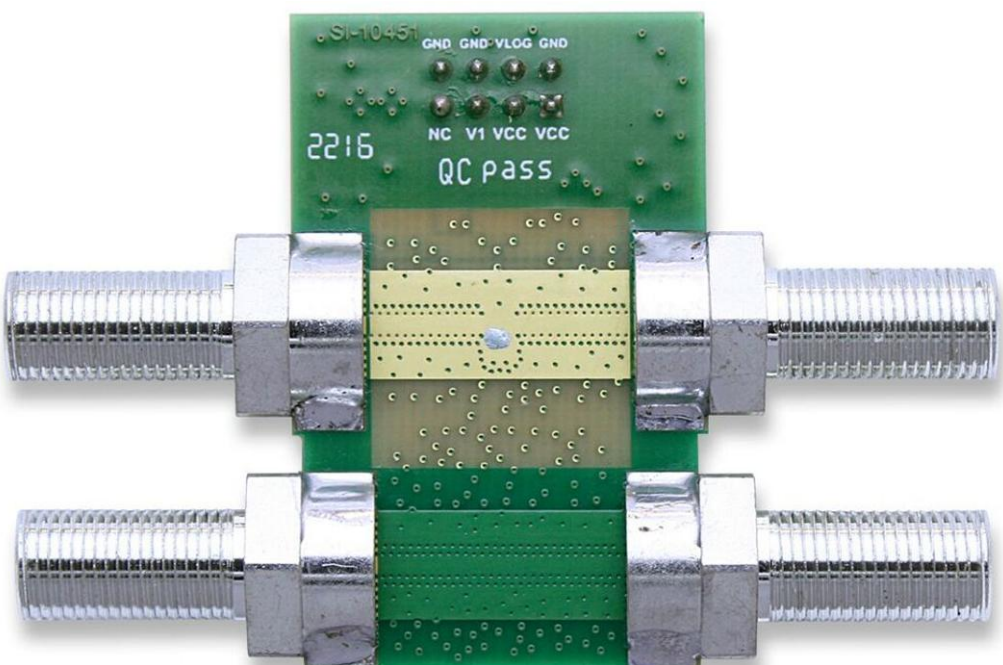
Figure 15. Bottom View
