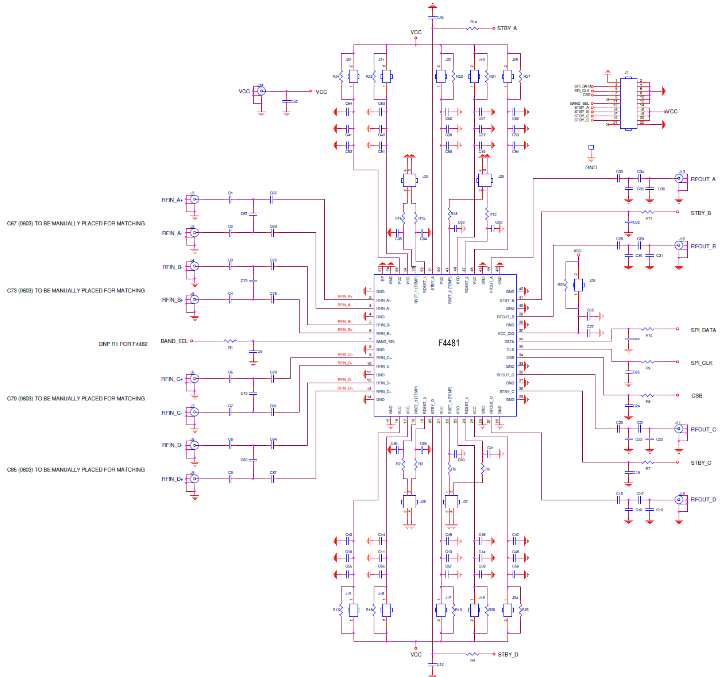
Figure 71. Applications Circuit
