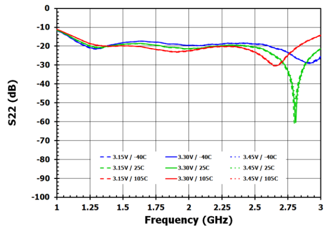
Figure 23. Output Return Loss at DSA = 14dB
