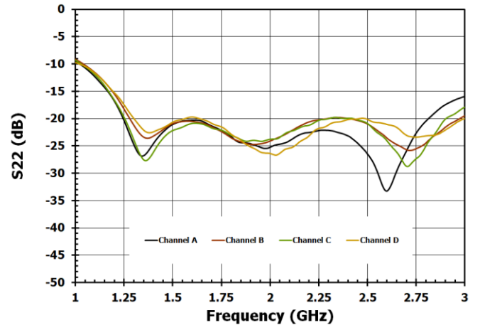
Figure 25. Output Return Loss vs Channel (DSA = 0dB)
