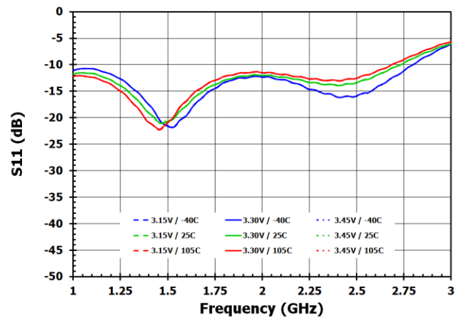
Figure 17. Input Return Loss at DSA = 14dB
