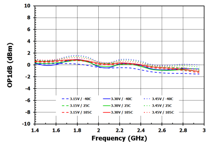
Figure 73. Band 2 OP1dB at DSA = 28dB
