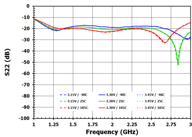
Figure 24. Output Return Loss at DSA = 31.5dB
