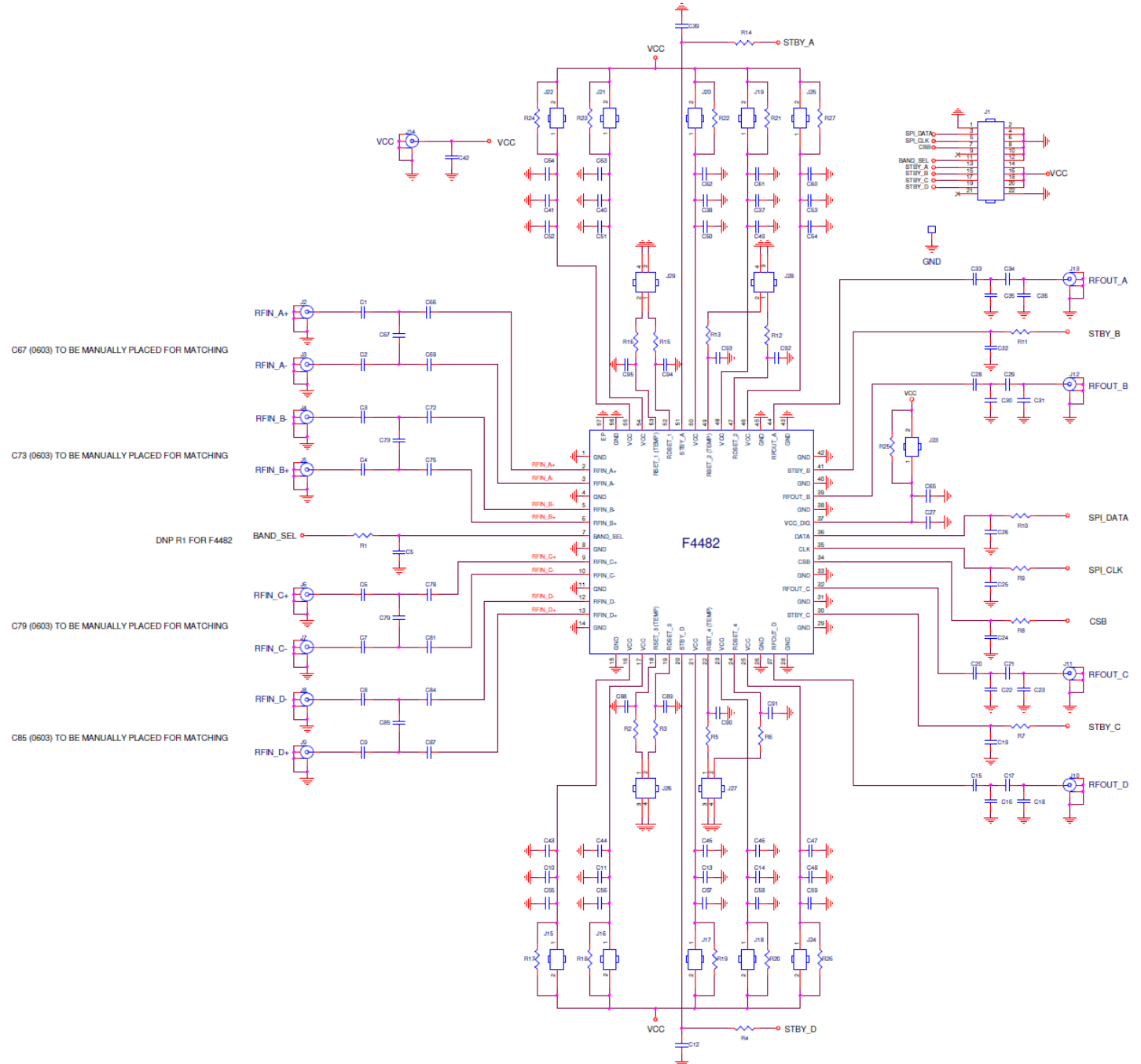
Figure 83. Electrical Schematic
