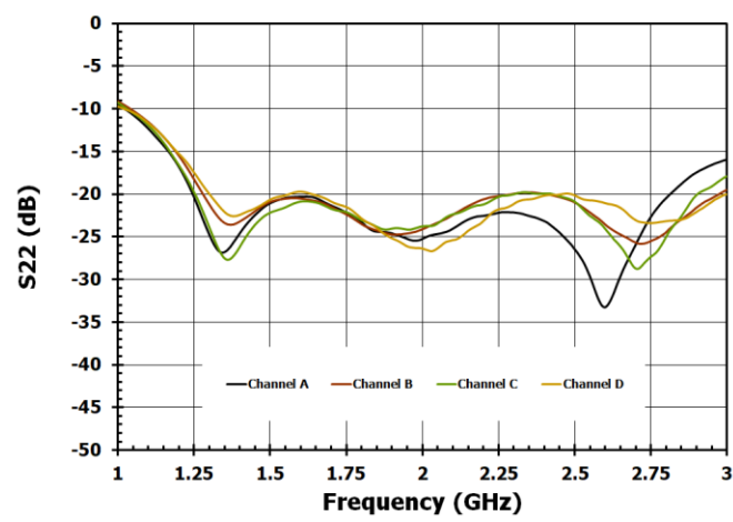
Figure 25. Output Return Loss vs Channel (DSA = 0dB)
