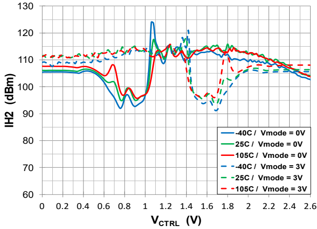
Figure 35. 2 nd Harmonic Input Intercept Point vs. V_{CTRL} over V_{MODE} and Temperature
