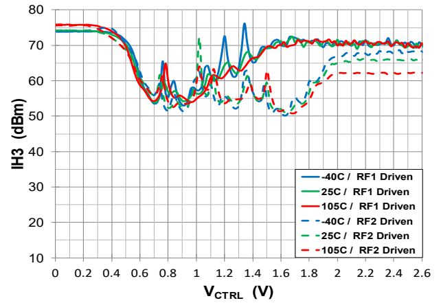
Figure 42. 3 rd Harm Input Intercept Point vs. V_{CTRL} over RF Port and Temp
