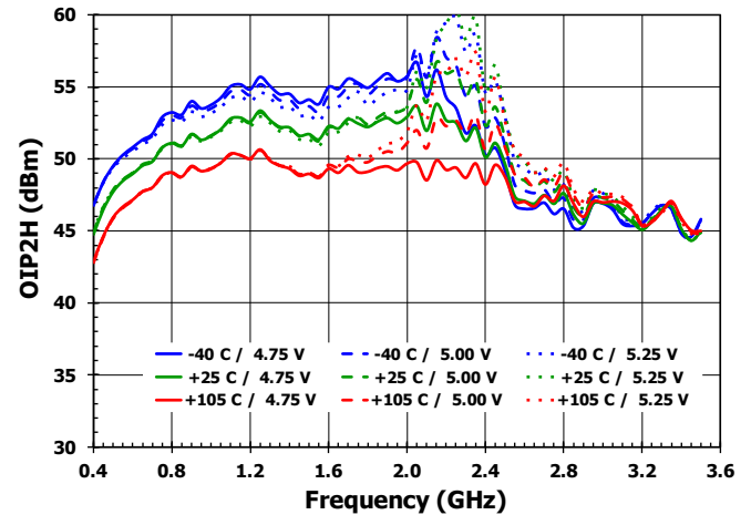
Figure 81. Output IP2H vs. Frequency over Temperature and Voltage – HB Mode
