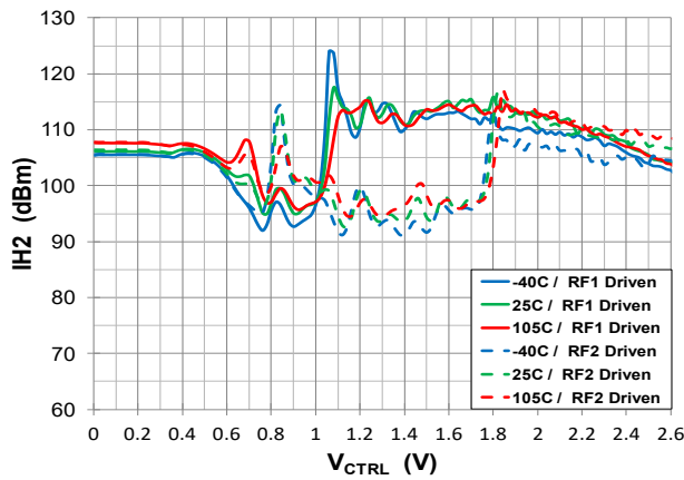
Figure 41. 2 nd Harm Input Intercept Point vs. V_{CTRL} over RF Port and Temp
