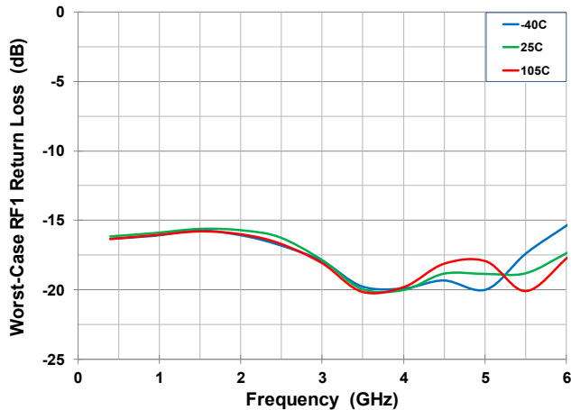
Figure 28. Worst-Case Return Loss (ATTEN_RF1 port) vs. Frequency over Temp
