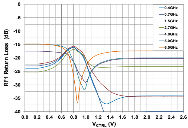
Figure 10. Return Loss (ATTEN_RF1 port) vs. V_{CTRL} over Frequency
