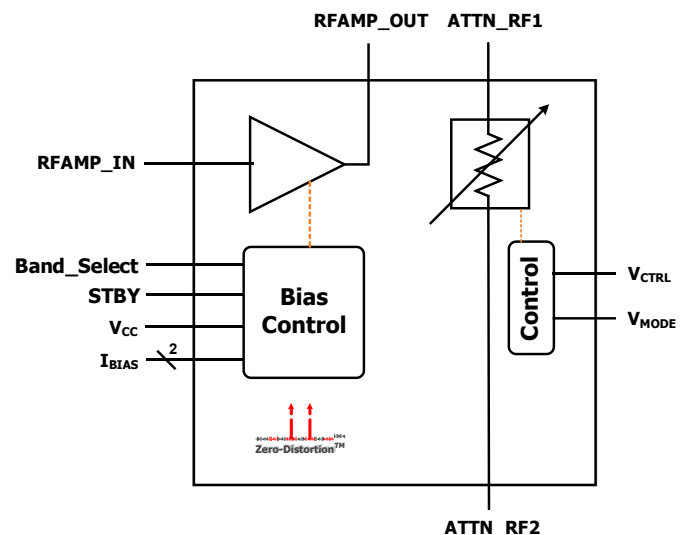
Figure 1. Block Diagram
