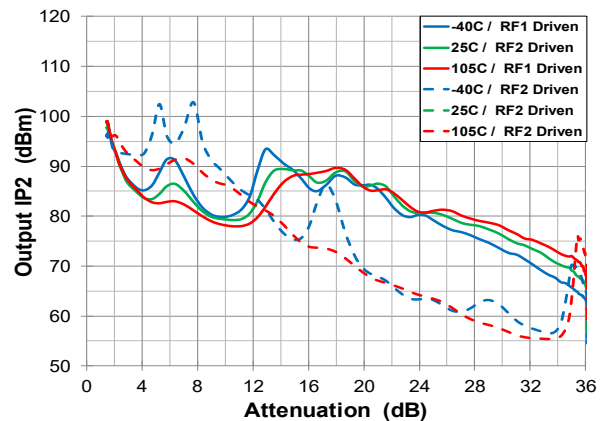
Figure 52. Output IP2 vs. Attenuation over RF Port and Temperature
