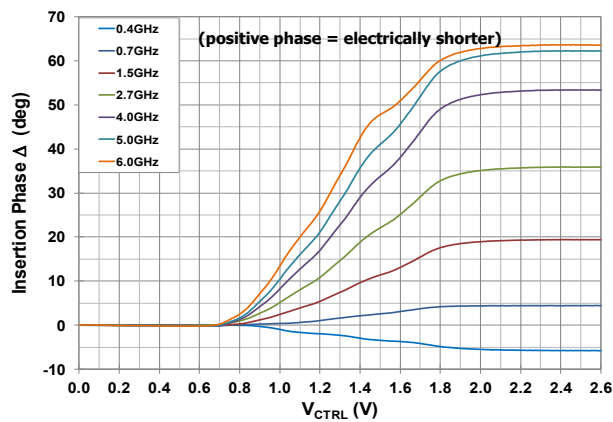
Figure 12. Insertion Phase Change vs. V_{CTRL} over Frequency
