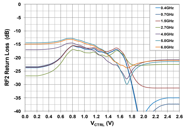
Figure 11. Return Loss (ATTEN_RF2 port) vs. V_{CTRL} over Frequency
