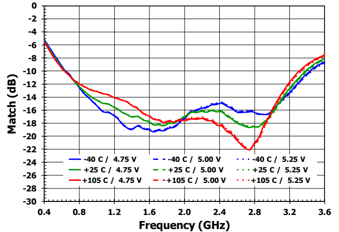
Figure 58. Output Match vs. Frequency over Temperature and Voltage – WB Mode
