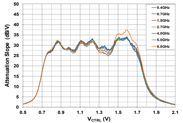
Figure 9. Attenuation Slope vs. V_{CTRL} over Frequency
