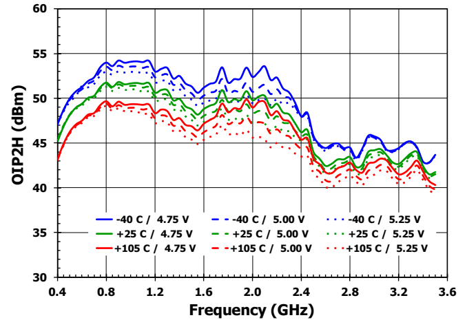
Figure 72. Output IP2H vs. Frequency over Temperature and Voltage – LB Mode
