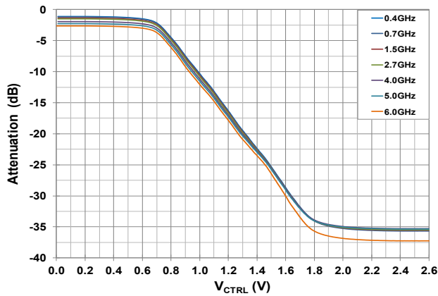
Figure 8. Attenuation vs. V_{CTRL} over Frequency
