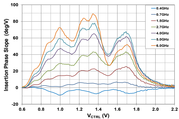
Figure 13. Insertion Phase Slope vs. V_{CTRL} over Frequency
