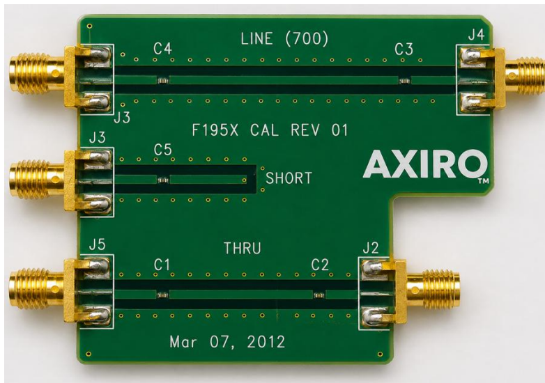
Standards used for F195x TRL calibration
