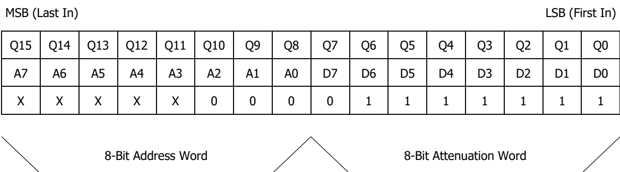
Figure 3. Default register settings set for max attenuation and 000 Address Word
