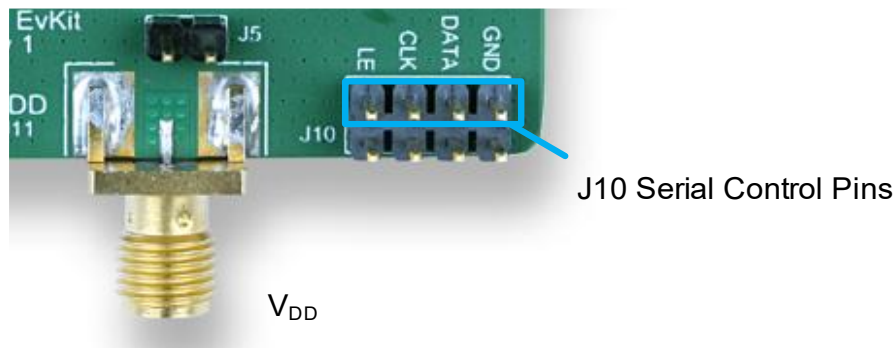
Figure 40. Serial Logic Connections
