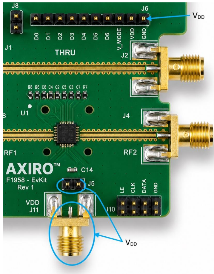
Figure 38. Power Supply Connections
