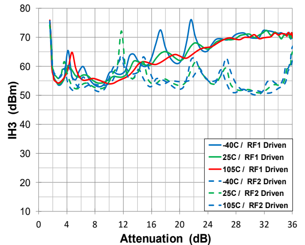
3 rd Harm Input Intercept Point vs. Attenuation
