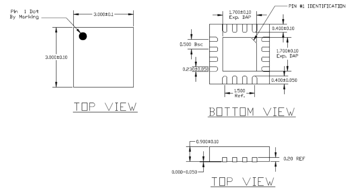
16LD QFN 3X3 (0.5MM PITCH)
