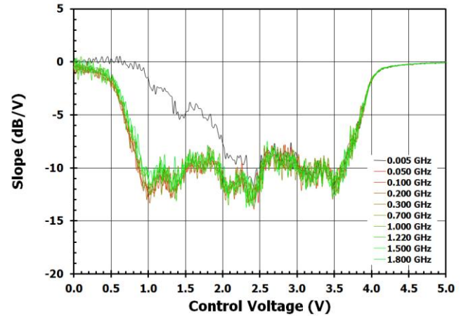
Figure 55. Attenuation Slope vs. V_{\text{CTRL}} [ V_{\text{MODE}} = \text{HIGH} ]
