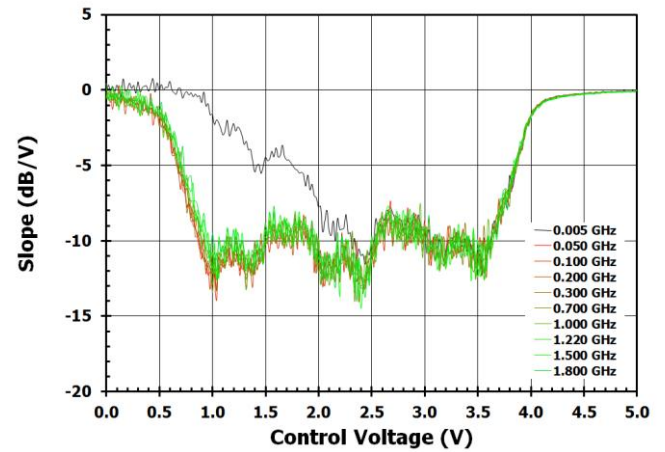
Figure 22. Attenuation Slope vs. V_{\text{CTRL}} [ V_{\text{MODE}} = \text{HIGH} ]
