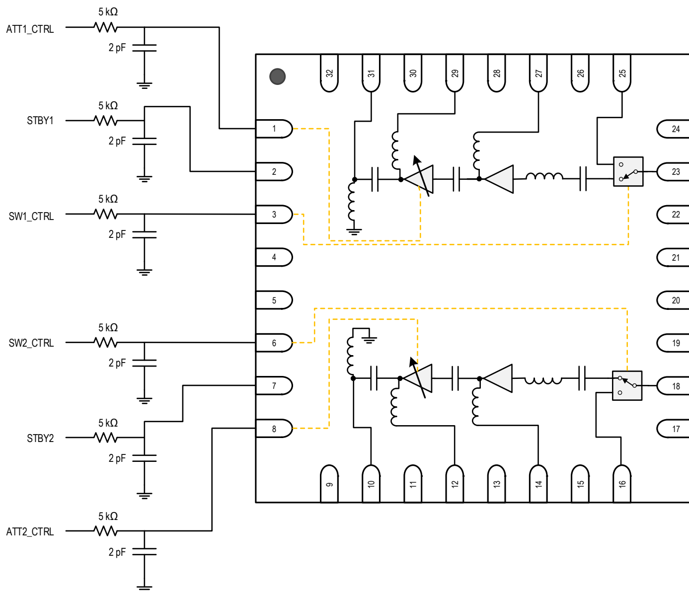
Figure 29. Control Pin Interface Schematic
