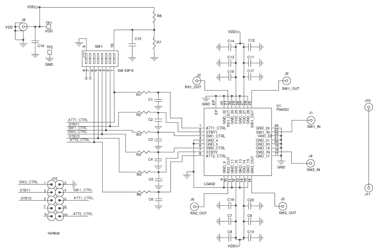
Figure 28. Electrical Schematic
