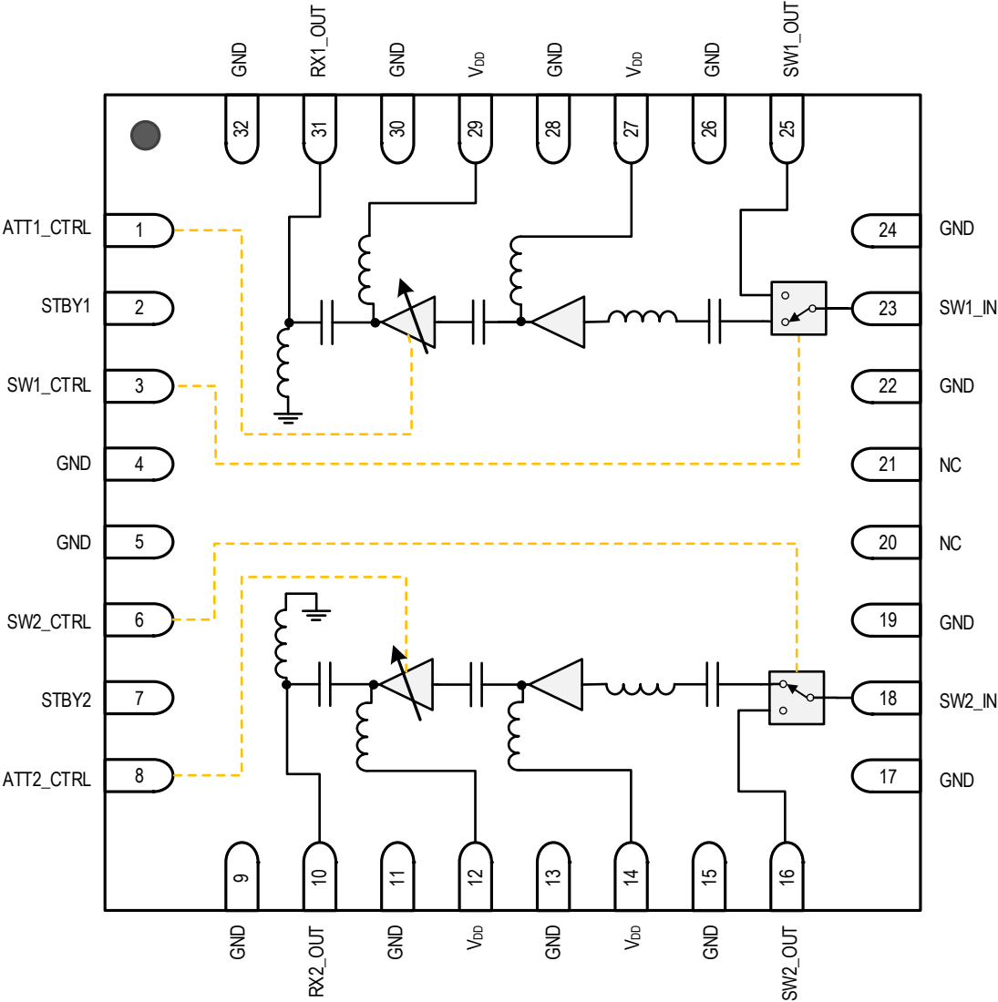
Figure 1. Pin Assignments for 6 × 6 × 0.75 mm 32-LGA – Top View
