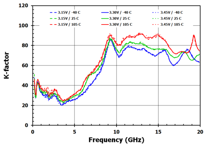
Figure 18. Stability K-factor
