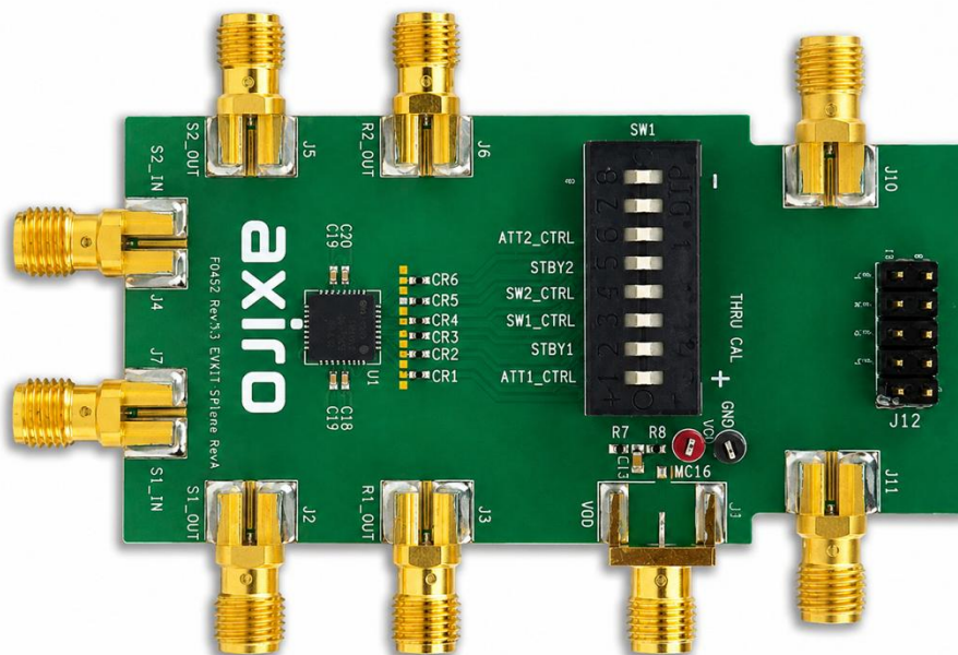
Figure 25. Evaluation Kit: Top View
