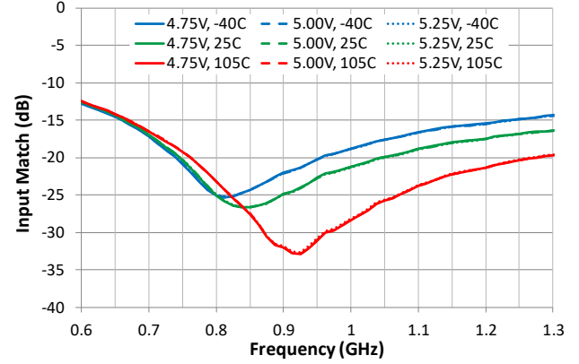
Input Match vs. Vcc and T CASE
