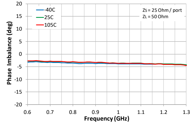
Phase Imbalance vs. T CASE
