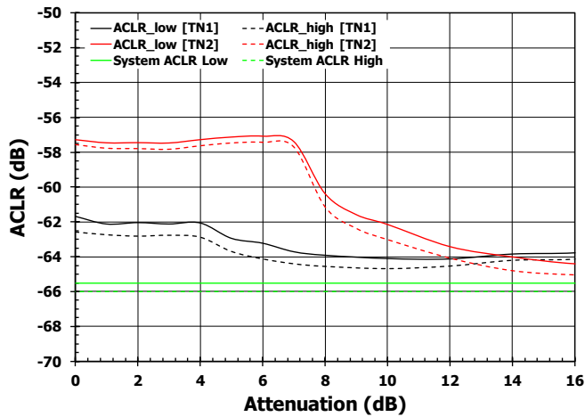
Figure 46. ACLR vs. Atten [1.88 GHz]
