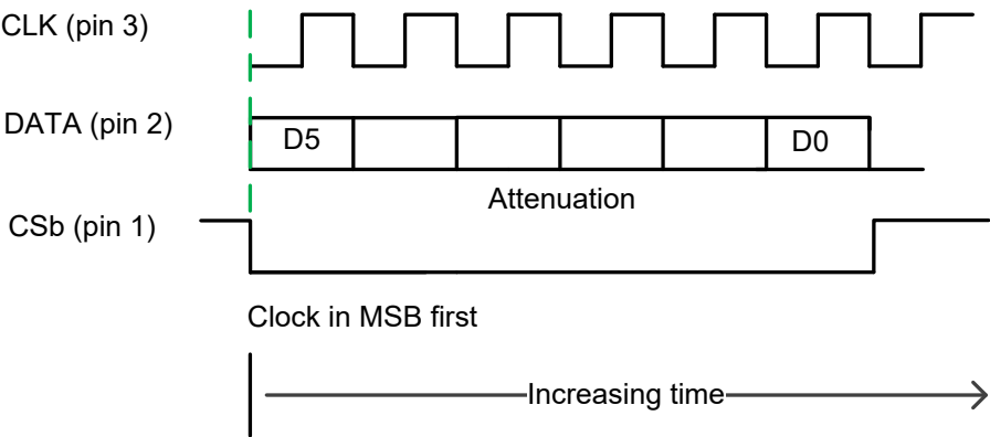
Figure 50. Serial Register Timing Diagram
