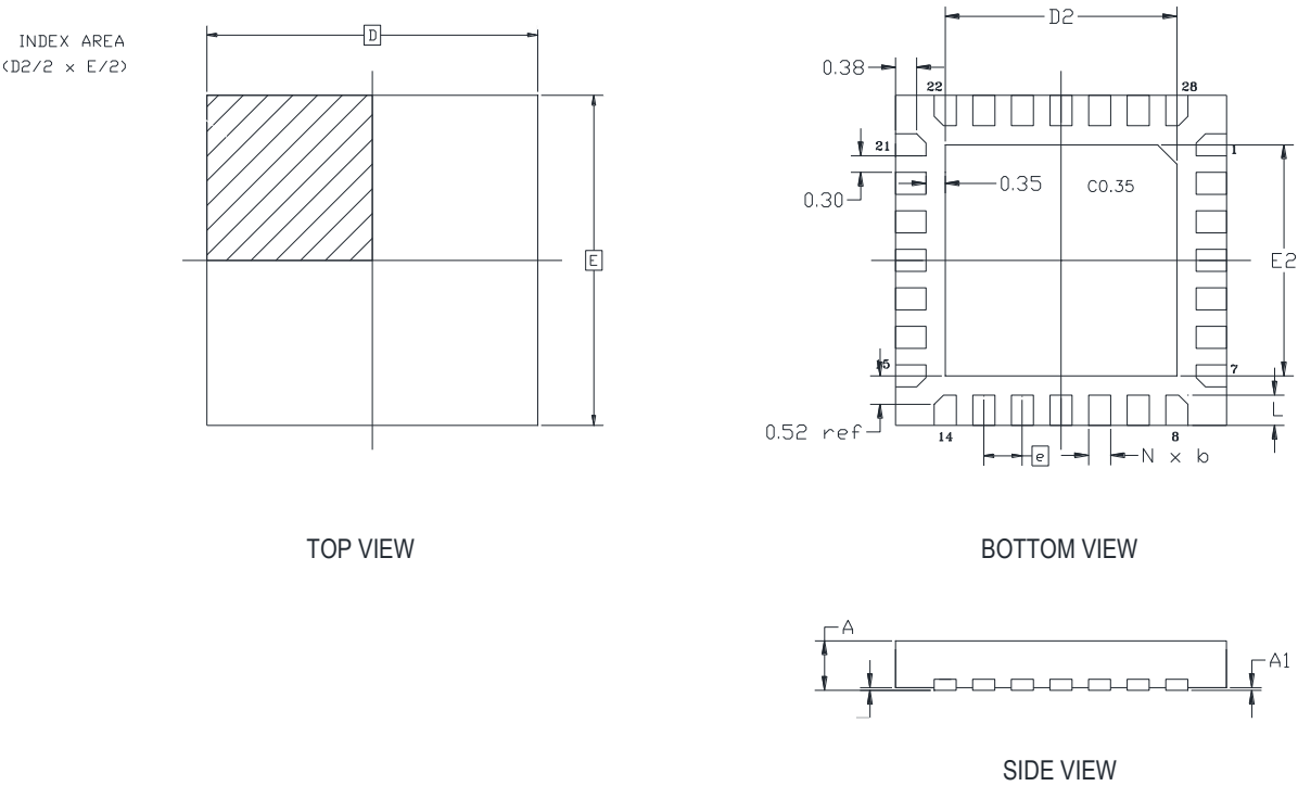
Figure 58. Package Outline Drawing NKG28 PSC-4606
