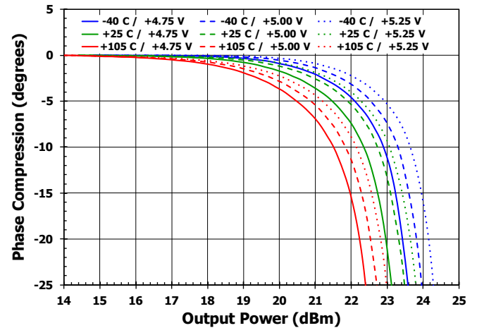
Figure 37. Phase Compression vs. Pout over Temp and Voltage [2.10 GHz]
