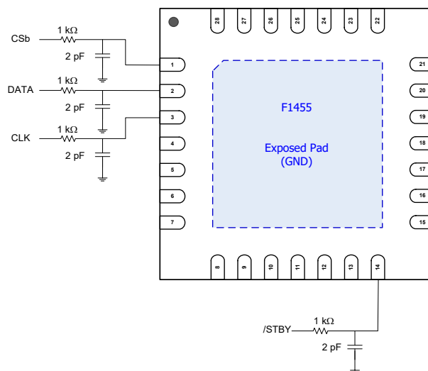
Figure 52. Control Pin Interface for Signal Integrity
