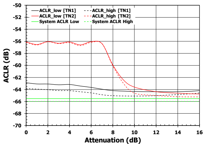
Figure 48. ACLR vs. Atten [2.10 GHz]
