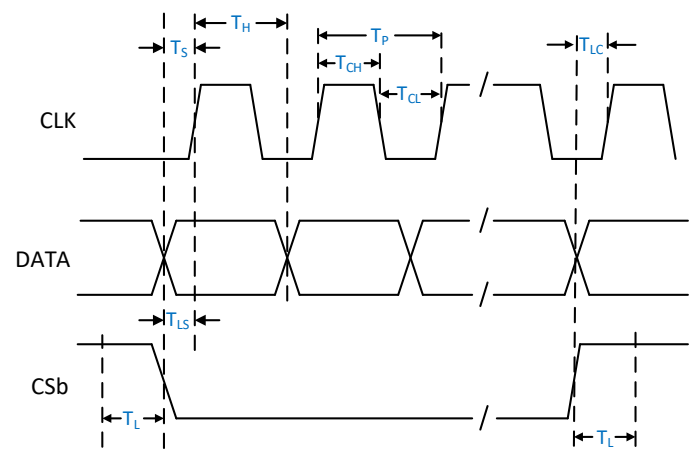
Figure 63. SPI Timing Diagram
