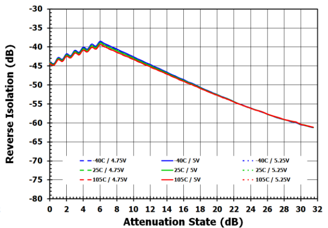
Figure 53. Reverse Isolation Vs. Attenuation [1.8GHz]
