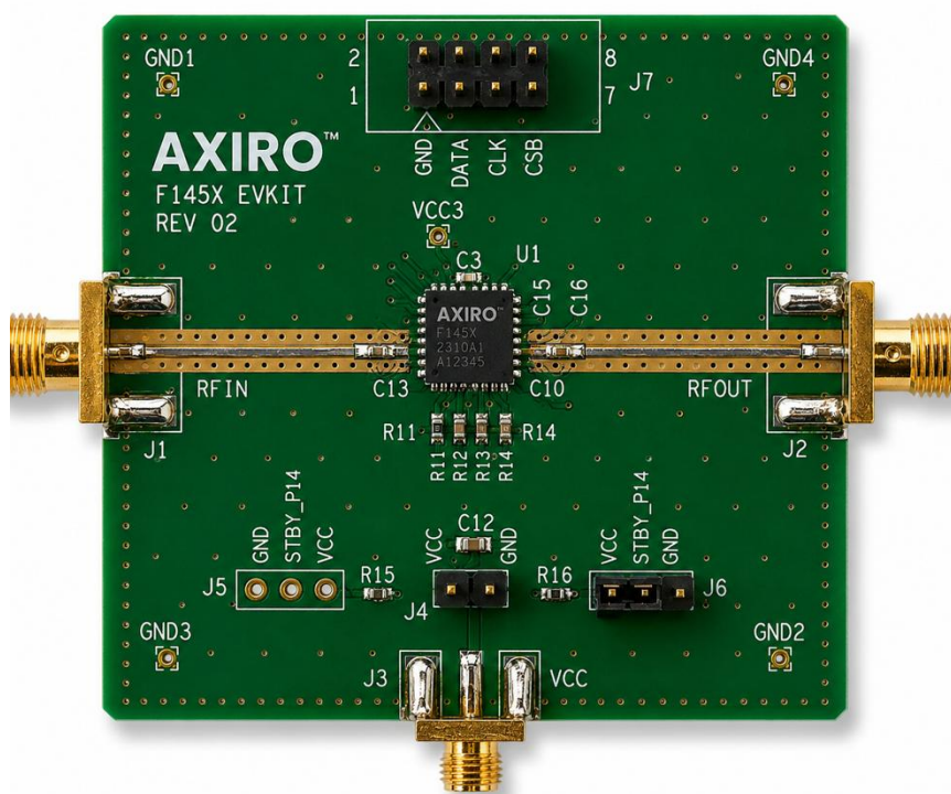
Figure 65. Top View
