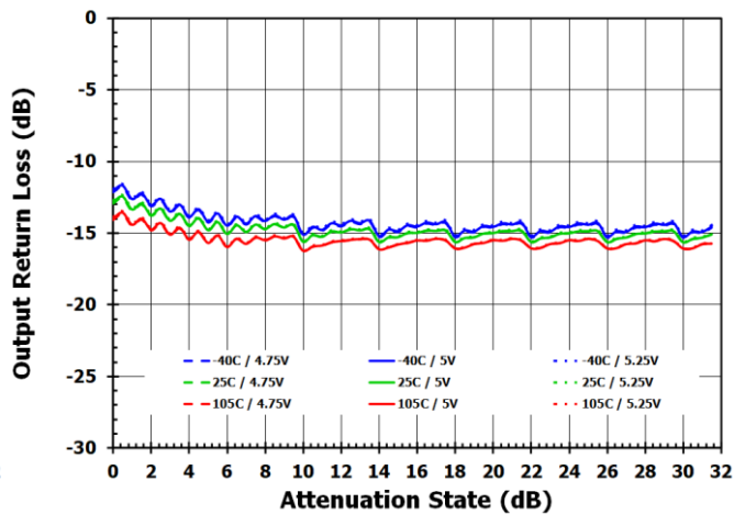
Figure 55. Output Return Loss Vs. Attenuation [1.8GHz]
