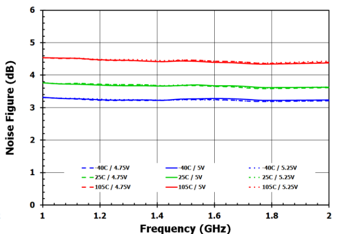
Figure 57. Noise Figure Vs. Frequency [Low Band]
