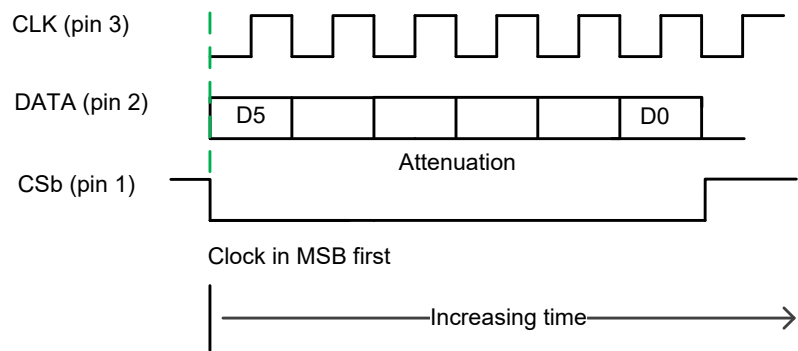
Figure 62. Serial Register Timing Diagram
