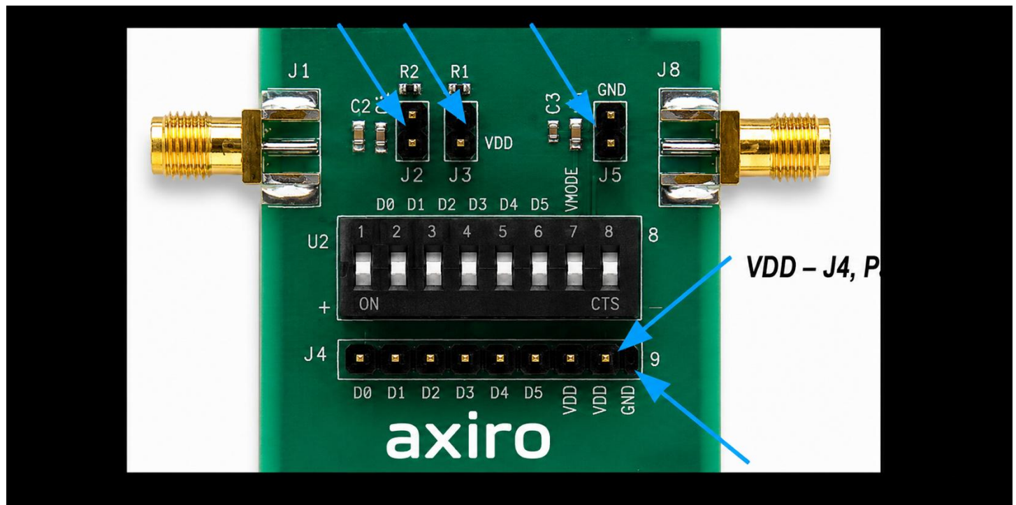
Figure 23. Power Supply and Logic Voltage Connections
