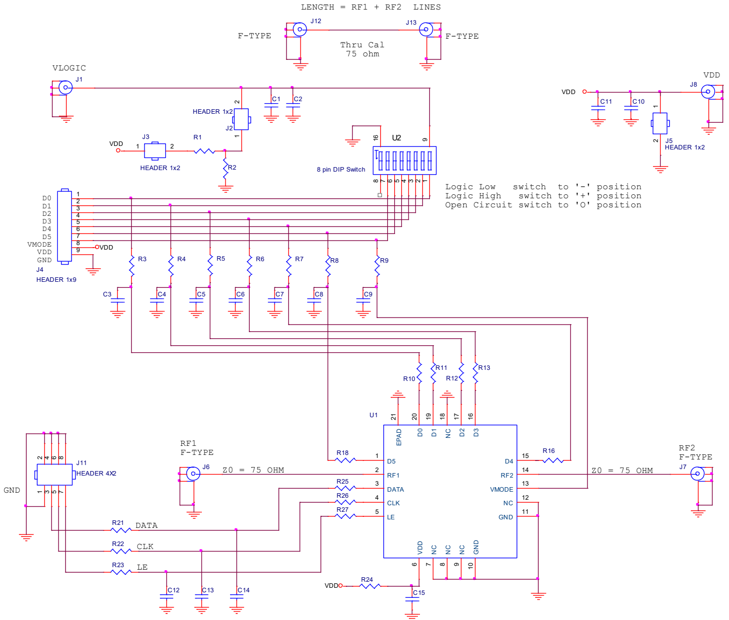
Figure 22. Electrical Schematic
