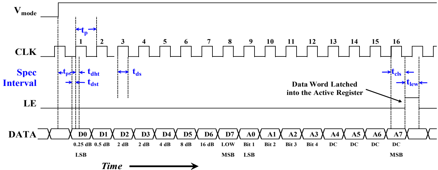
Figure 4 - Serial Timing Diagram
