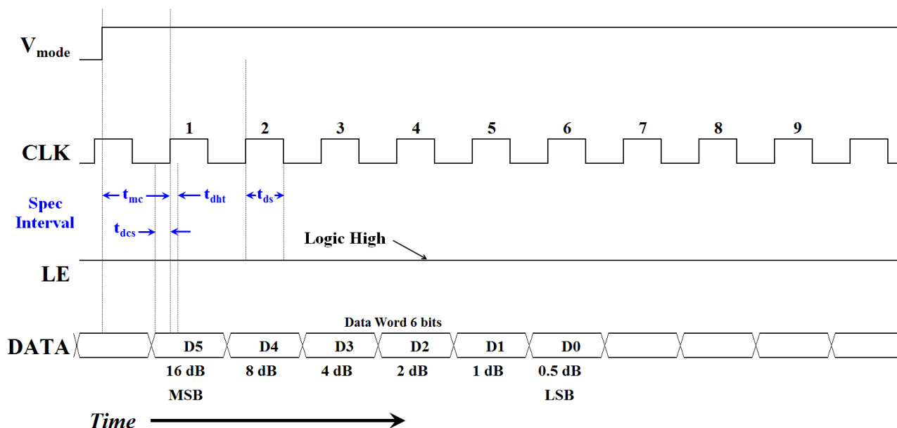
Figure 19. Direct Serial Register Timing Diagram
