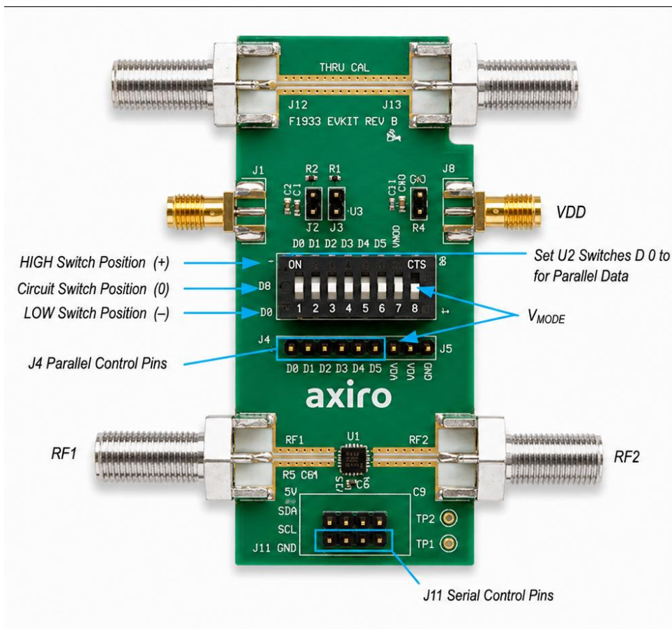
Figure 21. F1978EVB1 Evaluation Board – Top View
