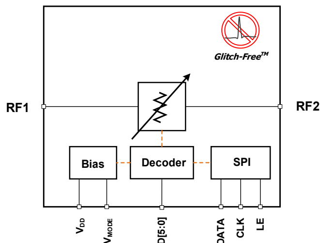
Figure 1. Block Diagram
