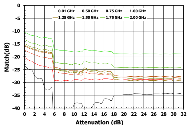
Figure 9. RF2 Return Loss vs. Attenuation State
