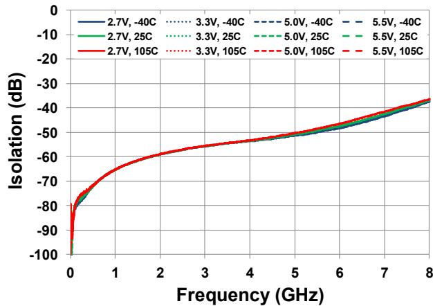
RF1 to RF2 Isolation [All Off State]
