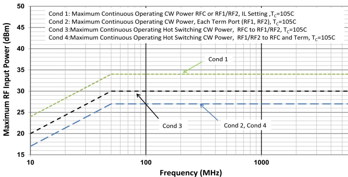
Figure 1: Maximum RF Input Operating Power vs. RF Frequency
